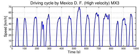
Fig. 8. High velocity driving cycle, c_3
